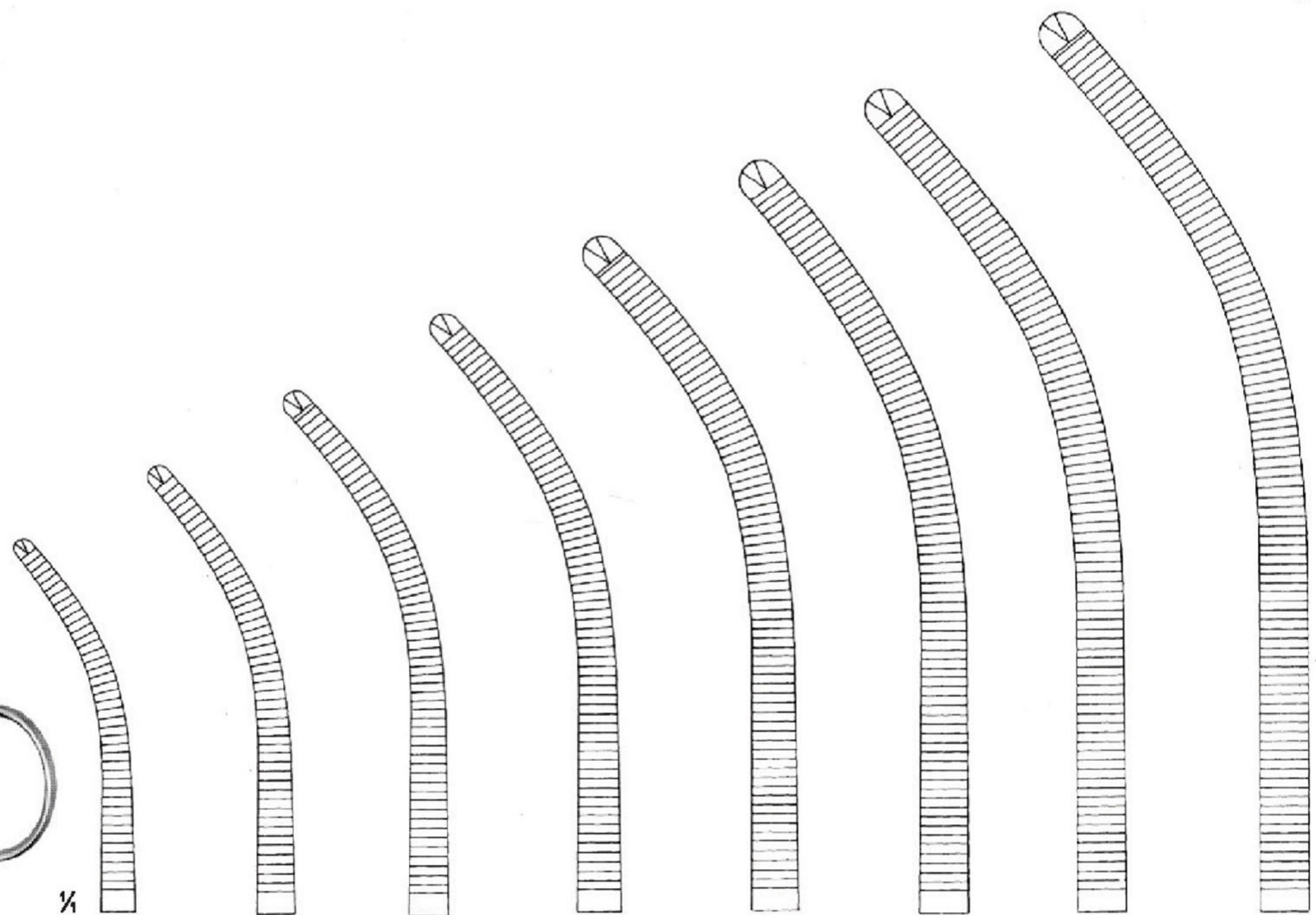
OI 11-2575-16 OI 11-2575-18 OI 11-2575-20 OI 11-2575-22 OI 11-2575-24 OI 11-2575-26 OI 11-2575-28 OI 11-2575-30 16 cm/6 1/4" 18 cm/7 1/8" 20 cm/7 7/8" 22 cm/8 1/2" 24 cm/9 1/2" 26 cm/10 1/4" 28 cm/11" 30 cm/11 3/4"
